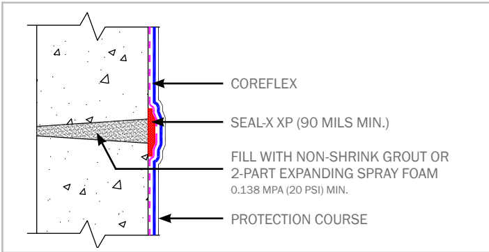
TAPER TIE
