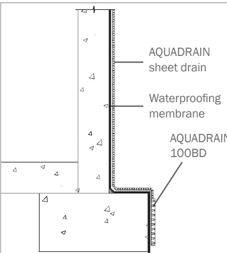
FOUNDATION WALL
