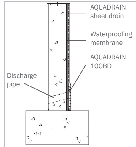
RETAINING WALL
